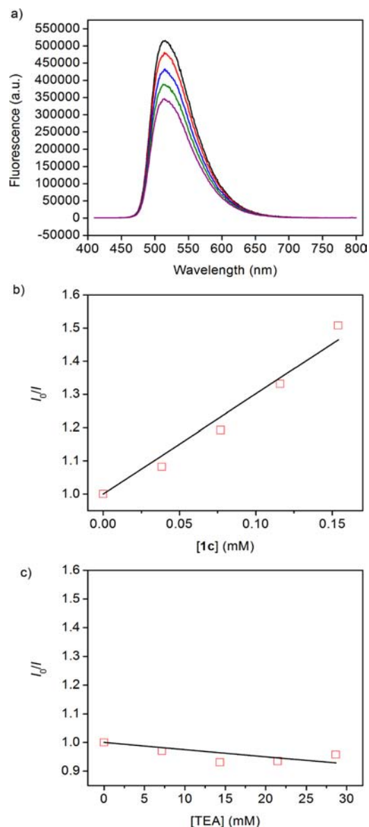
Figure 8. (a) Fluorescence spectra of an acetonitrile solution containing 0.05 mM Ir(ppy) 3 in the absence (black) and presence of 0.04 mM (red), 0.08 mM (blue), 0.12 mM (green), and 0.15 mM (purple) 1c . (b) Linear plots of ratio of fluorescence intensities in the absence and presence of 1c versus the concentration of (b) 1c ( y = 3021x + 1 , R^2 = 0.97 ) and (c) TEA, according to the Stern–Volmer equation.
