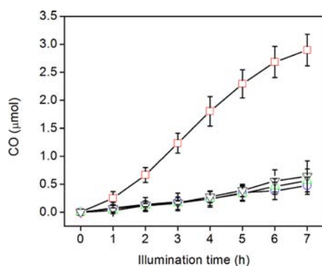
Figure 5. Photocatalytic reduction of CO 2 to CO in a 0.07 M TEA acetonitrile solution containing 0.2 mM Ir(ppy) 3 (black triangles), 0.2 μM 1c (blue circles), 0.2 mM Ir(ppy) 3 and 0.2 μM Ni-(CH 3 CN) 4 (PF 6 ) 2 (green triangles), and 0.2 mM Ir(ppy) 3 and 0.2 μM 1c (red squares), using a 130 mW·cm -2 Xe lamp fitted with an AM 1.5 filter.
