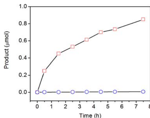
Figure 4. \text{CO} (red squares) and \text{CH}_4 (blue circles) formation vs. electrolysis time in a controlled potential electrolysis in a 0.1 M \text{NBu}_4\text{PF}_6 acetonitrile solution containing 2 \mu\text{M} 1c at -1.8 \text{ V vs SCE} using a glassy carbon disk electrode under a \text{CO}_2 atmosphere.
