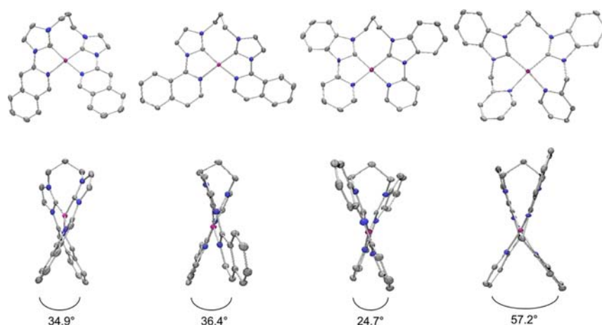
Figure 1. Solid-state structures of 1c–4c (left to right). The top row shows a front view; the bottom row provides a side view, highlighting the torsional twist induced by ligand flexibility. Anions, solvent molecules, and hydrogen atoms are omitted for clarity; thermal ellipsoids are shown at 50% probability.
