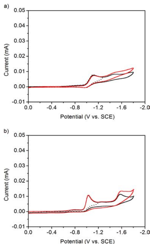
Figure 3. Cyclic voltammograms of complex (a) 4c and (b) 5c in a 0.1 M \text{NBu}_4\text{PF}_6 acetonitrile solution under a \text{N}_2 (black) and \text{CO}_2 (red) atmosphere using a glassy carbon disk electrode at a scan rate of 100 \text{ mV}\cdot\text{s}^{-1} .
