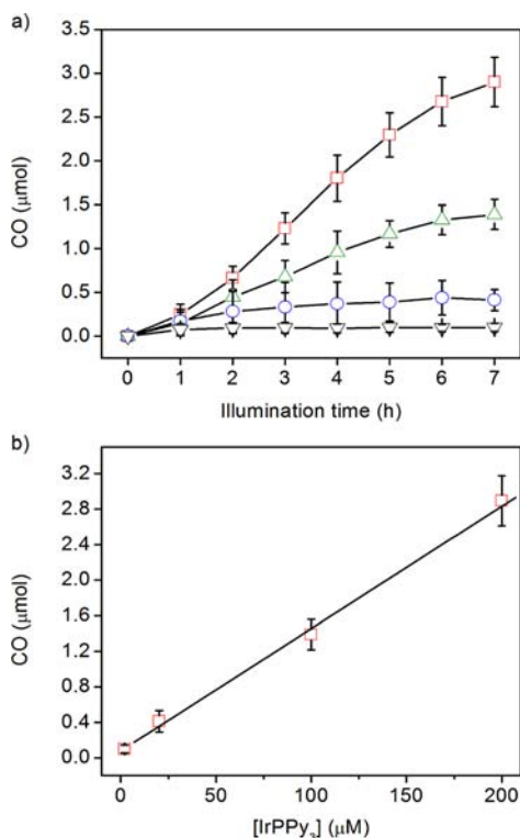
Figure 7. (a) Photocatalytic reduction of CO 2 to CO in a 0.07 M TEA acetonitrile solution containing 0.2 μM 1c and 0.2 mM (red squares), 0.1 mM (green triangles), 0.02 mM (blue circles), and 0.002 mM (black triangles) Ir(ppy) 3 , using a 130 mW·cm -2 Xe lamp fitted with an AM 1.5 filter. (b) Linear plot of CO production at the end of 7 h versus Ir(ppy) 3 concentration.
