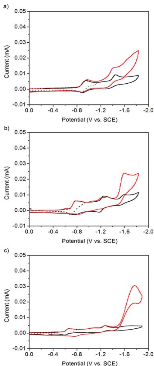
Figure 2. Cyclic voltammograms of complexes (a) 1c , (b) 2c , and (c) 3c in a 0.1 M \text{NBu}_4\text{PF}_6 acetonitrile solution under a \text{N}_2 (black) and \text{CO}_2 (red) atmosphere using a glassy carbon disk electrode at a scan rate of 100 \text{ mV}\cdot\text{s}^{-1} .
